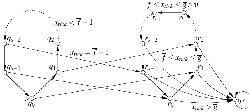
Fig. 3. The FCADBMs for the formula \forall i. f \le i \le g \wedge i \equiv_s t \rightarrow v
